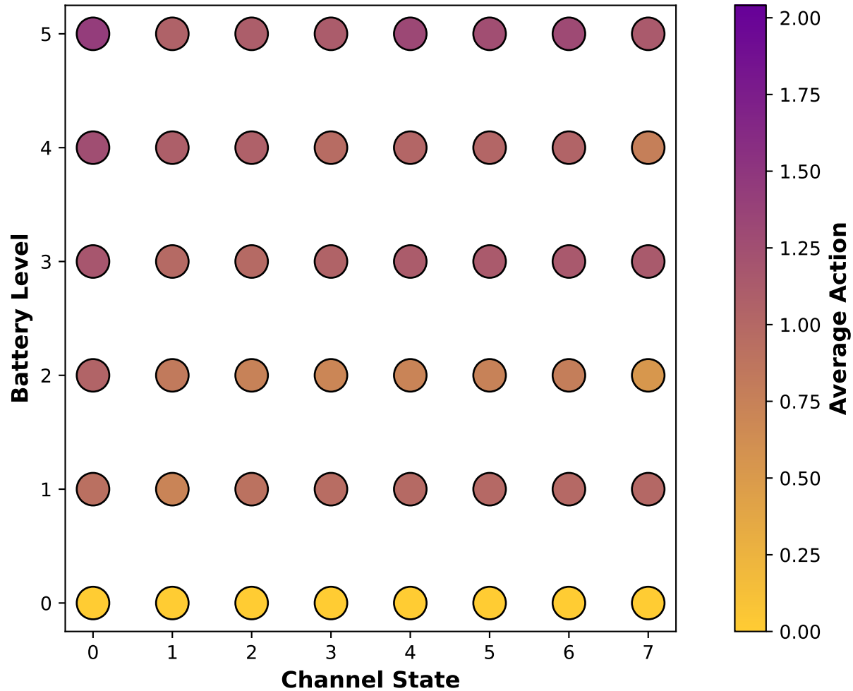
JAL: Scatter Action Map
